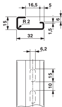
Dimensioned drawing
