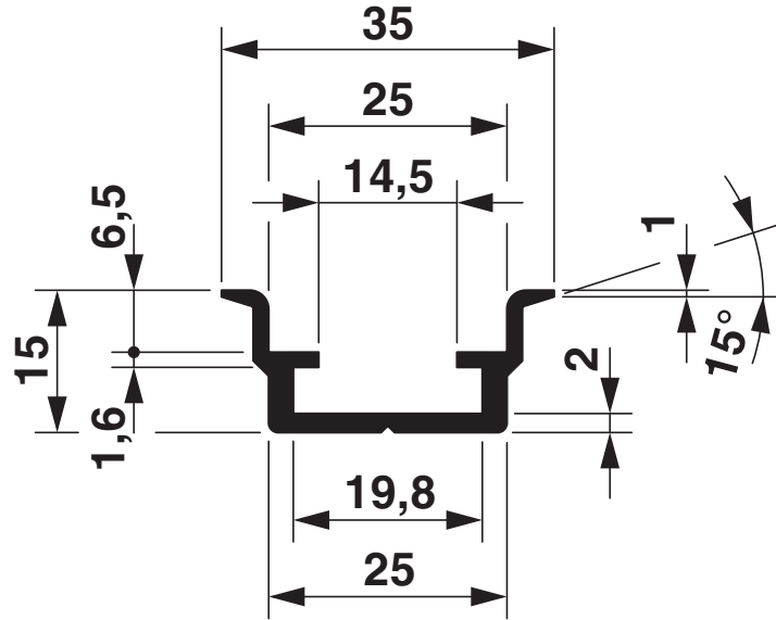
Dimensioned drawing
