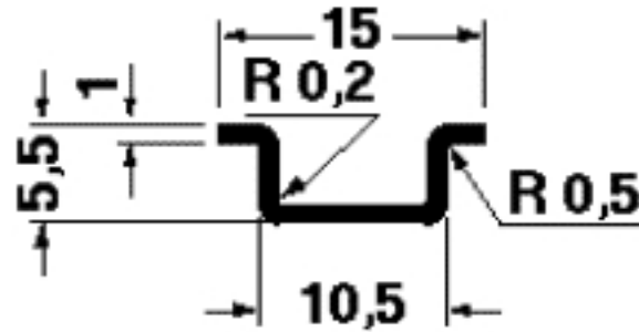
Dimensioned drawing
